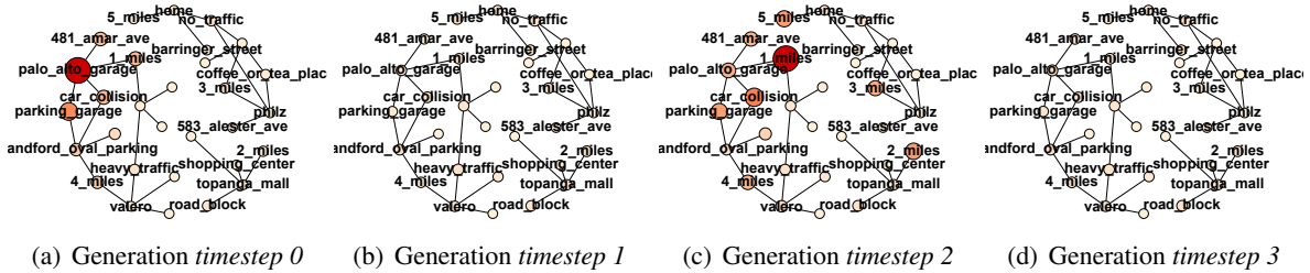
Figure 5: Knowledge graph attention visualization when generating responses in the SMD navigation domain. Based on the question “Where is a nearby parking garage?”, the generated response of our model is “palo_alto_garage is 1_miles away”. Specifically, the attention results at each generation timestep for the knowledge graph information of this example are shown in (a), (b), (c) and (d) respectively. The color and size of the nodes represent their attention weights. The darker and bigger the nodes are, the larger their attention weights are. Our model successfully learns to attend to the correct KB entities (i.e., palo_alto_garage and 1_miles at generation timesteps 0 and 2) which have the highest attention, and the model copies them to serve as the output words. During timesteps 1 and 3, the model generates output words (i.e., is and away ) from the vocabulary.
